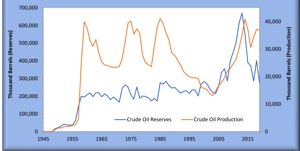
Figure 3.2 - Utah Crude Oil Production and Total Proved Reserves, 1945-2019
