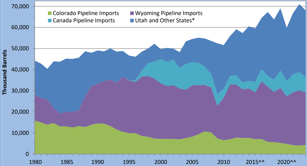
Figure 3.8 - Utah Refinery Receipts of Crude Oil by State of Origin, 1980-2023
