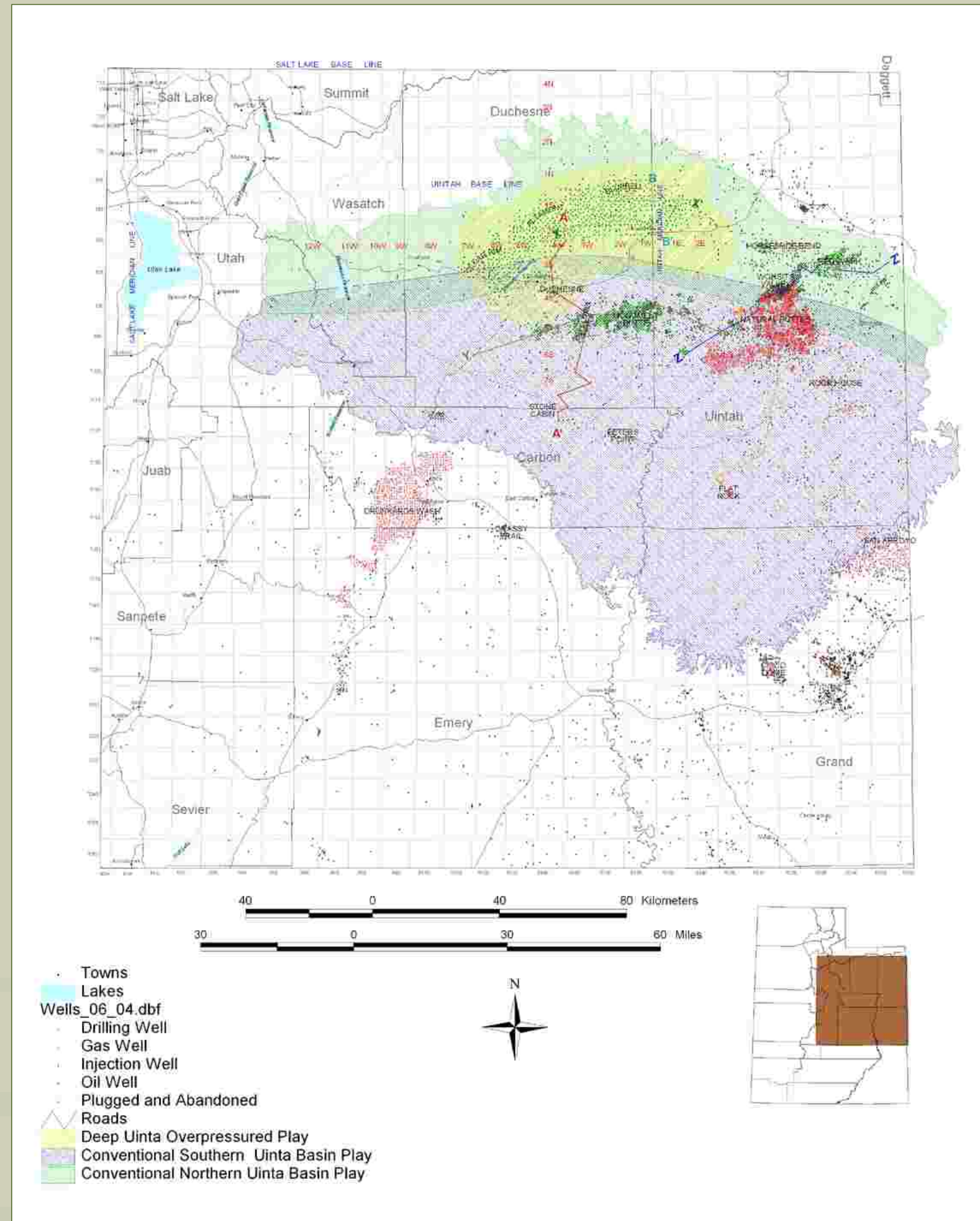
Uinta Basin location map showing boundaries (overlapping) of the Green River petroleum plays. Dashed line is the approximate limit where reservoir temperature is above pour-point temperature of the oil.
