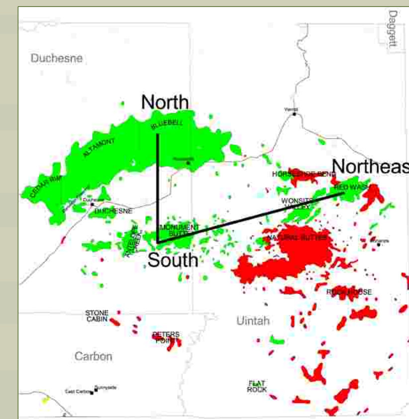
Location of diagrammatic correlation line.
