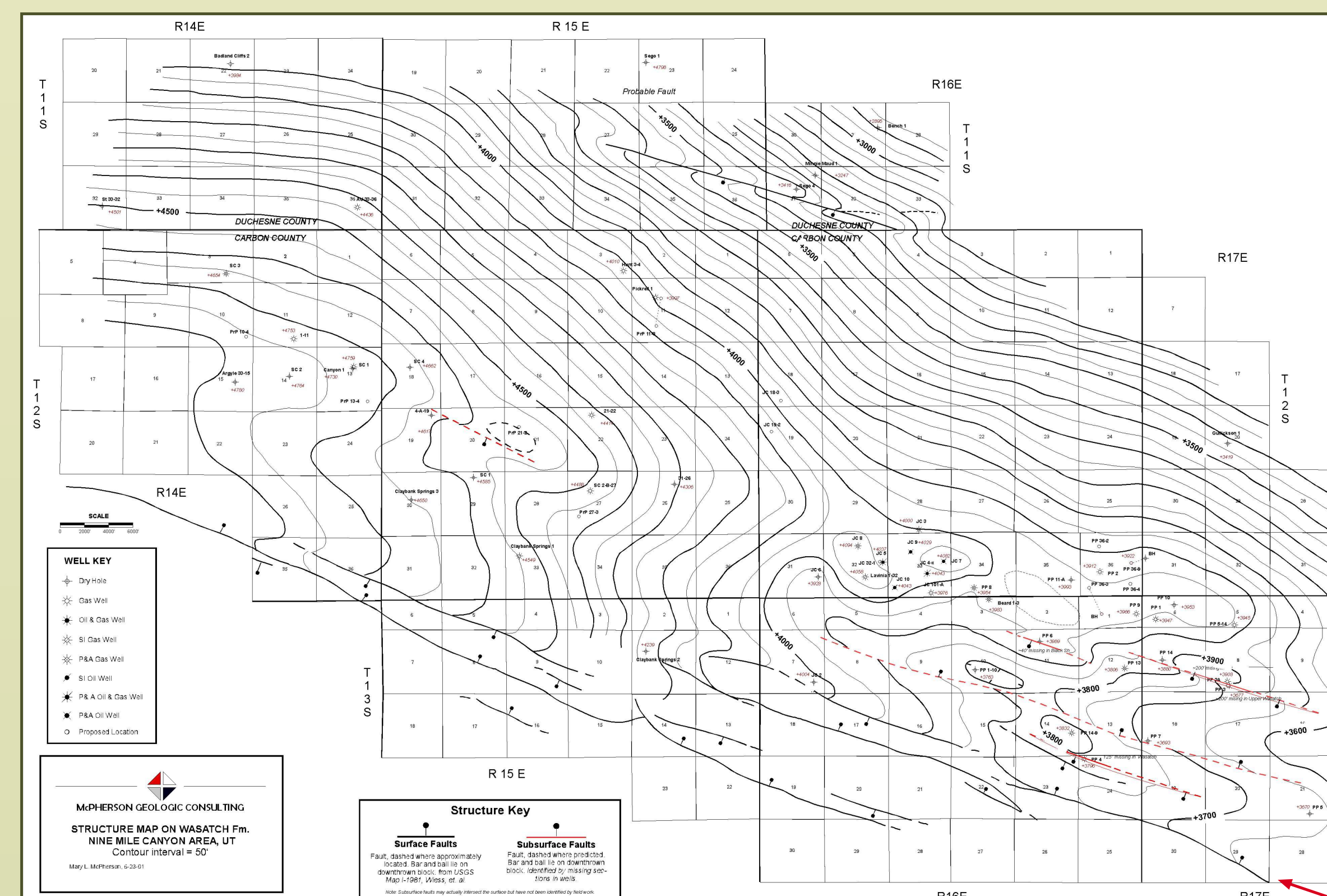
Structure contour map of the Peters Point (Jack Canyon) - Stone Cabin fields.
