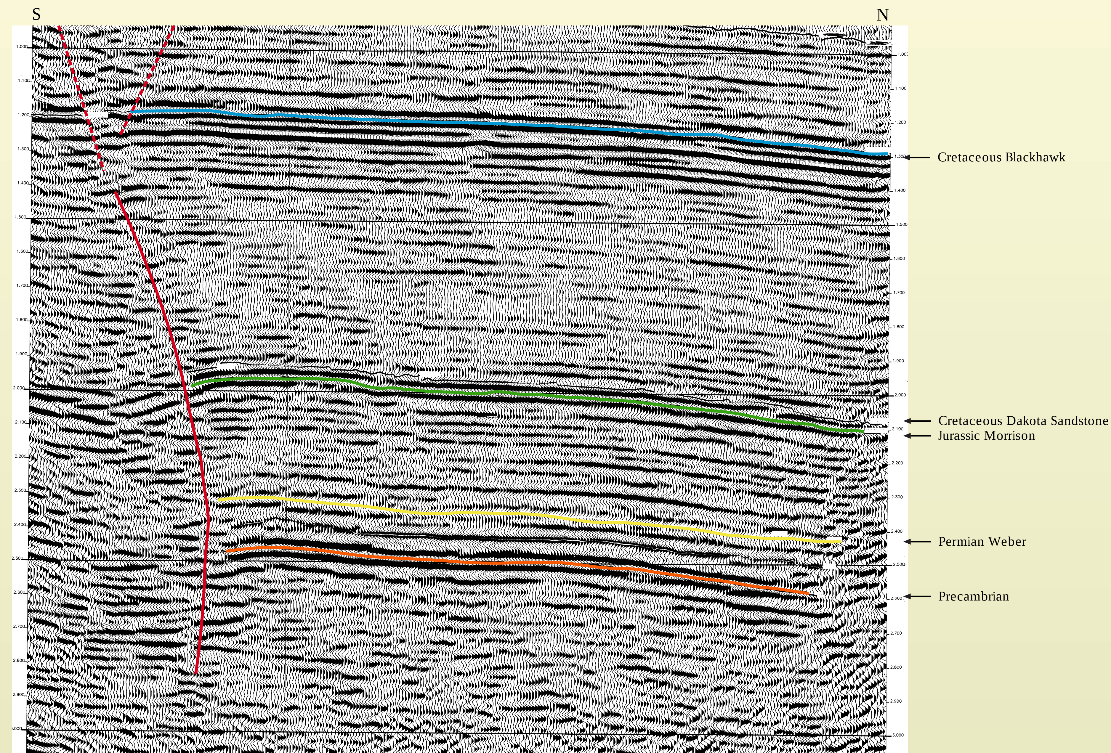
Seismic profile across the Peters Point anticline
