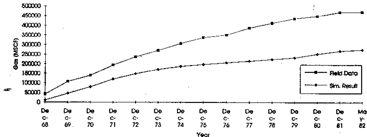
Figure 55. Actual versus simulated cumulative gas production of the lower Green River Formation/upper Wasatch transition from three wells in the four-square mile (10.4 km 2 ) west study-site (sections 9, 10, 15, and 16, T. 1 S., R. 2 W.).
