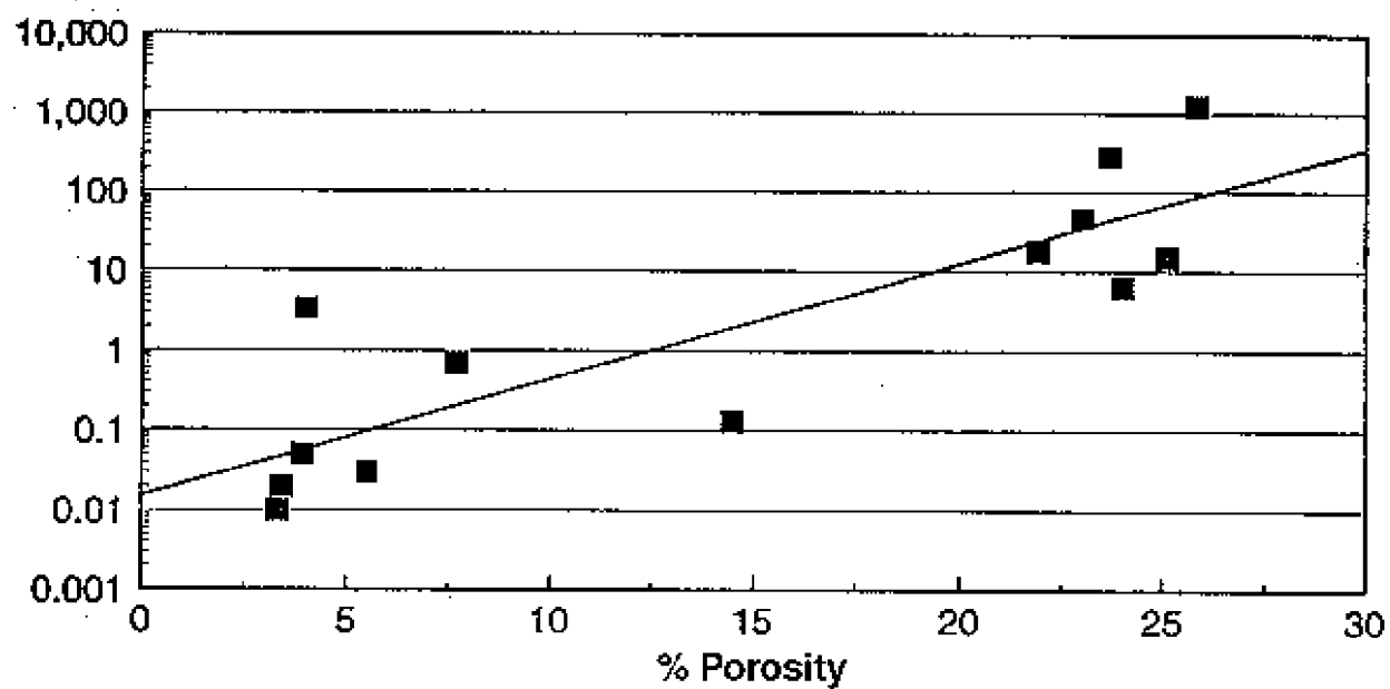
Figure 30. Porosity (percent) versus horizontal permeability (millidarcies) of core-plug samples classified as arenites.
