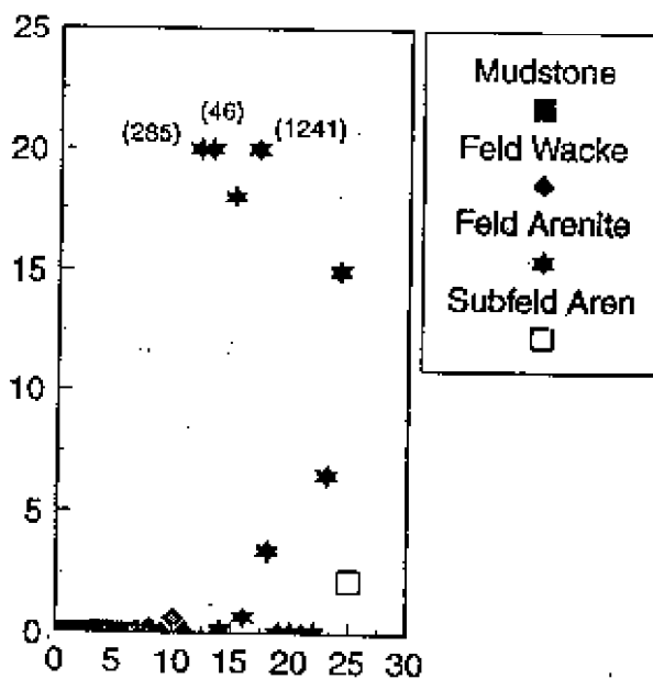
Figure 29. Porosity of clastic core-plug samples taken from the outcrop (the vertical axis is percent porosity, the horizontal is the number of samples) compared to the horizontal permeability (the vertical axis is millidarcies of permeability, the horizontal is the number of samples).
