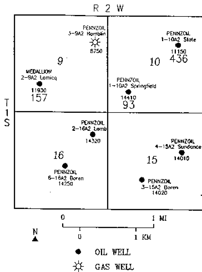
Figure 23. Cumulative oil production, in thousands of barrels, from the lower Green River Formation.
