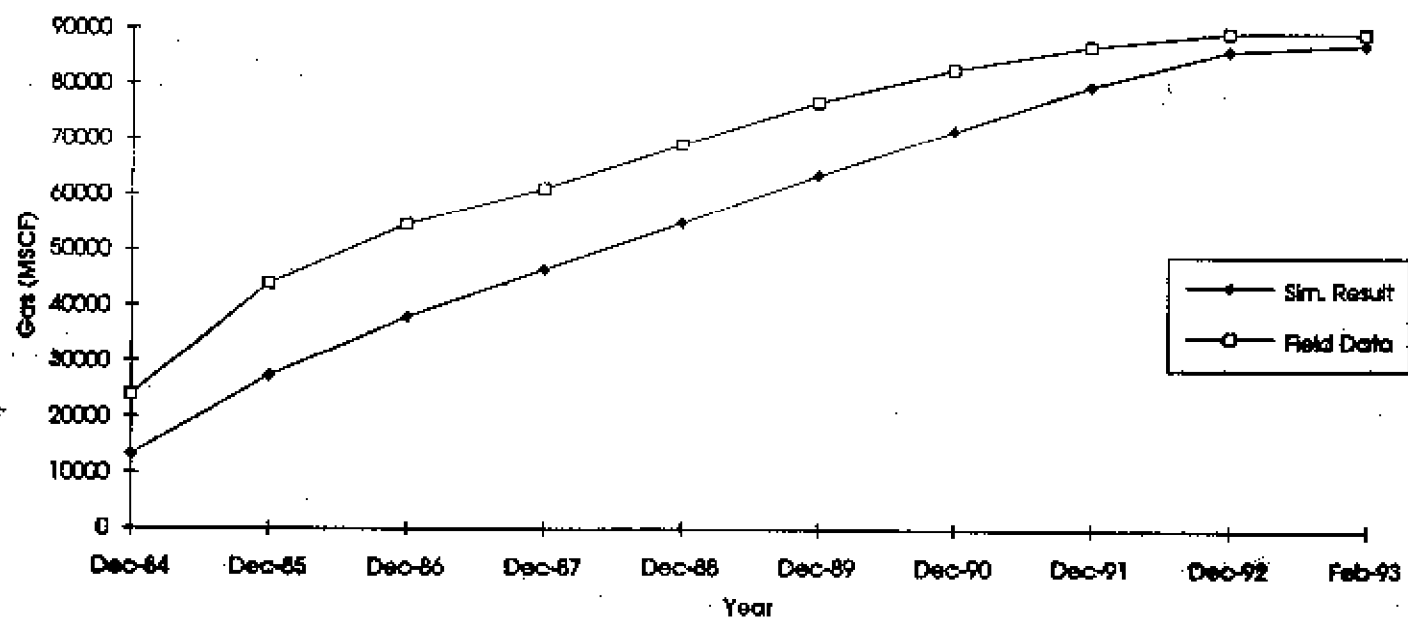
Figure 43. Actual versus preliminary single-well model simulated cumulative gas production for the Michelle Ute well.
