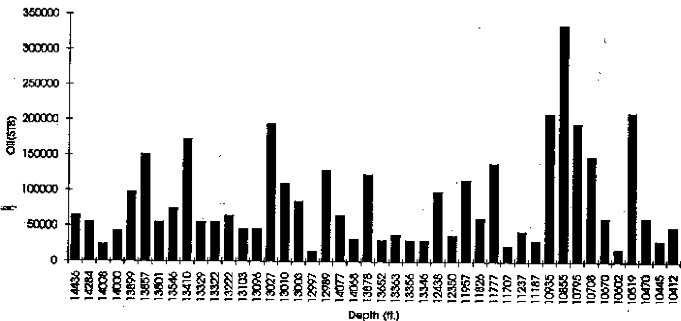
Figure 39. Original oil-in-place calculations for all perforated zones in the Michells Ute well.
