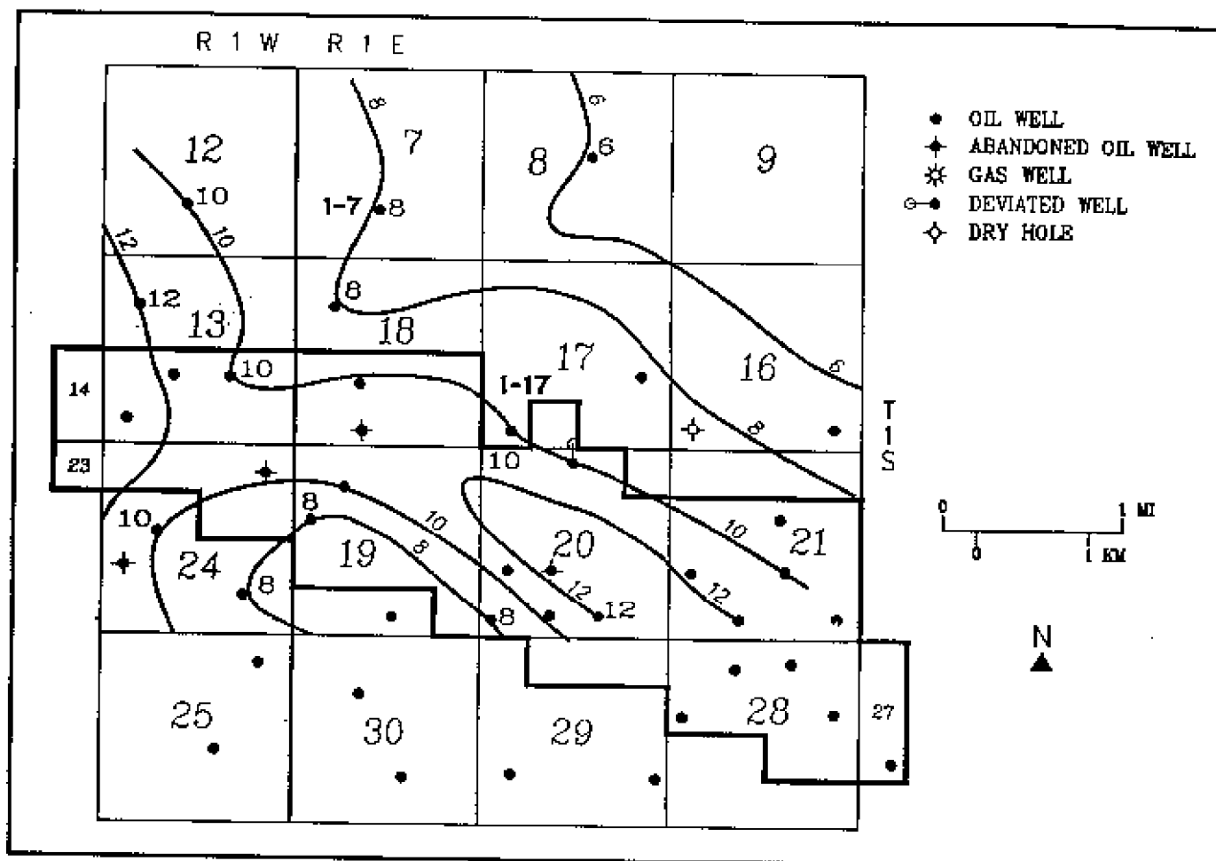
Figure 17. Thickness map of the GEL-4 bed. Contour interval is 2 feet.
