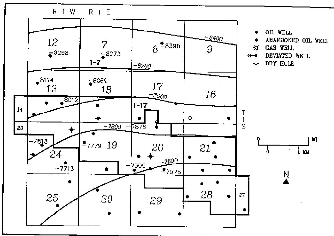
Figure 20. Structure contour map of the top of the OEL-3 bed. Contour interval is 200 feet.
