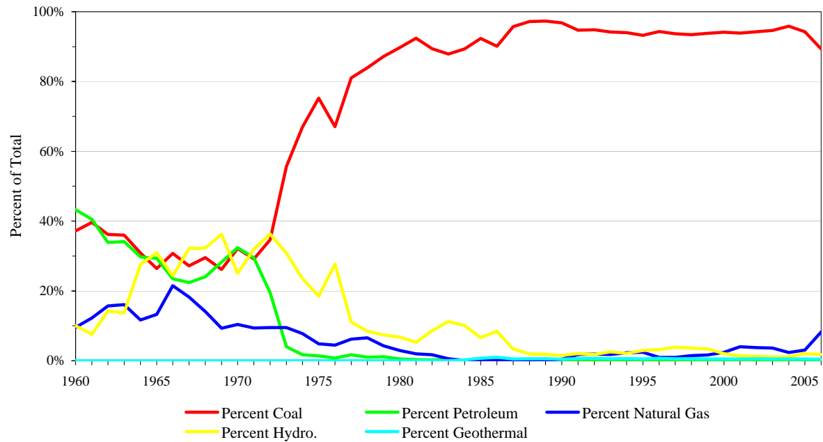
Figure 1.5b - Net Generation of Electricity in Utah by Energy Source, 1960-2006
