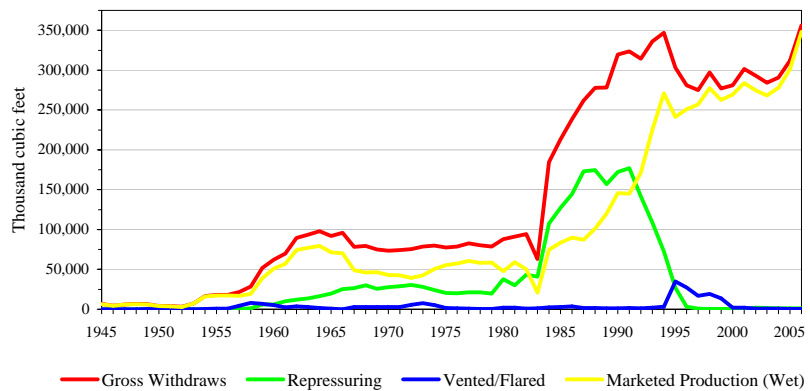
Figure 4.3 - Gross Withdrawal and Marketed Production of Natural Gas in Utah, 1945-2006
