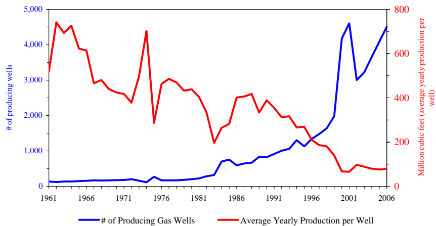
Figure 4.4 - Average Yearly Natural Gas Production per Well in Utah Verses the Number of Producing Wells, 1961-2006
