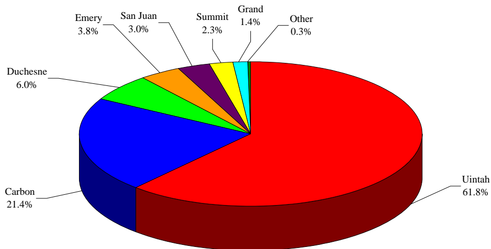
Figure 4.5 - Natural Gas Gross Production in Utah by County, 2008
