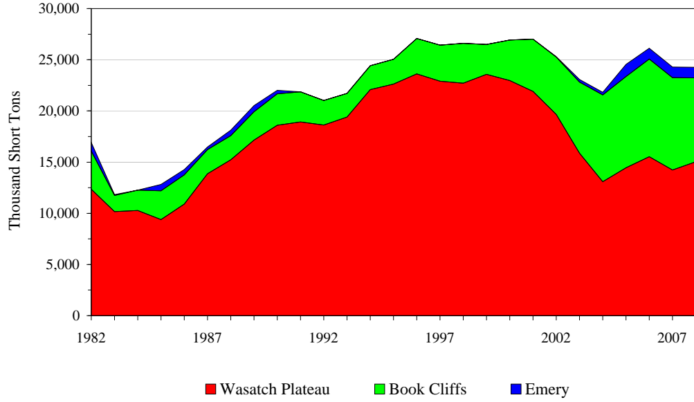
Figure 2.3 - Coal Production in Utah by Coal Field, 1982-2008
