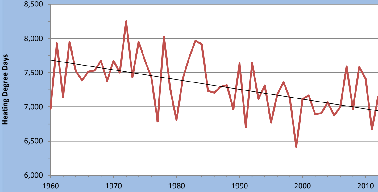
Figure 7.2 - Heating Degree Days in Utah, 1960-2016
