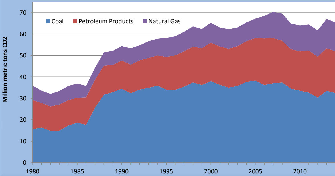
Figure 8.1 - Carbon Dioxide Emissions in Utah by Energy Source, 1980-2014
