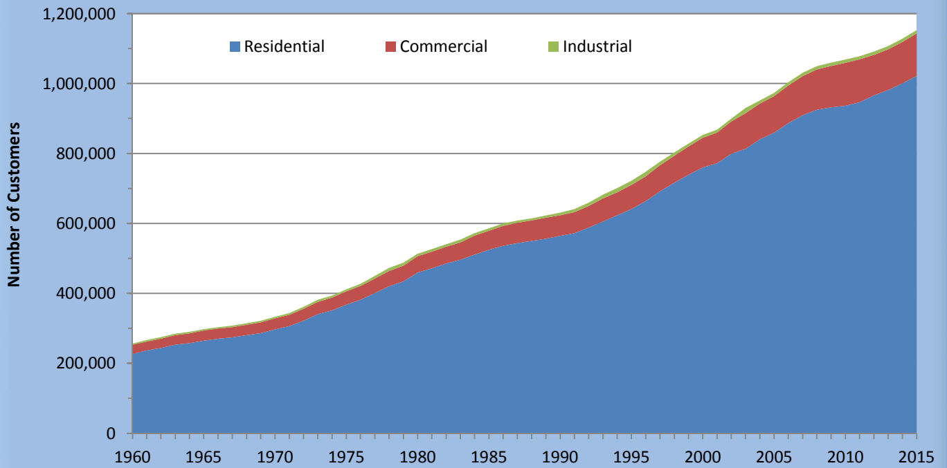
Figure 5.7 - Electric Utility Customers in Utah by Class of Service, 1960-2015
