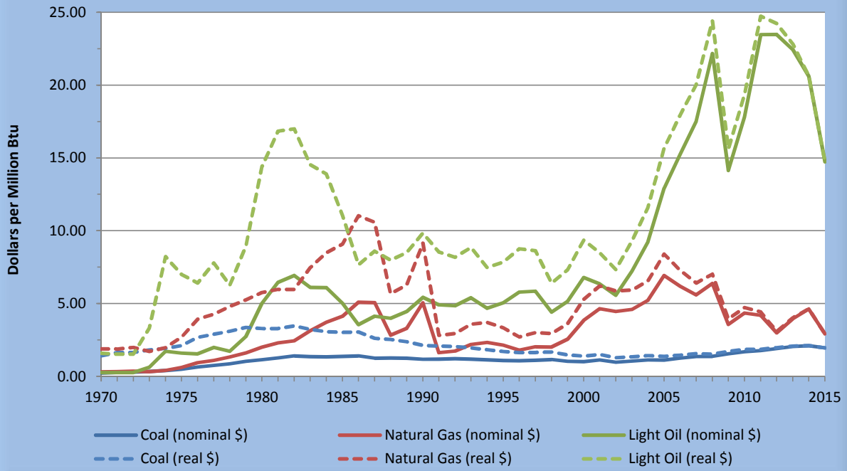
Figure 5.3 - Cost of Fuel to Generate Electricity in Utah, 1970-2015
