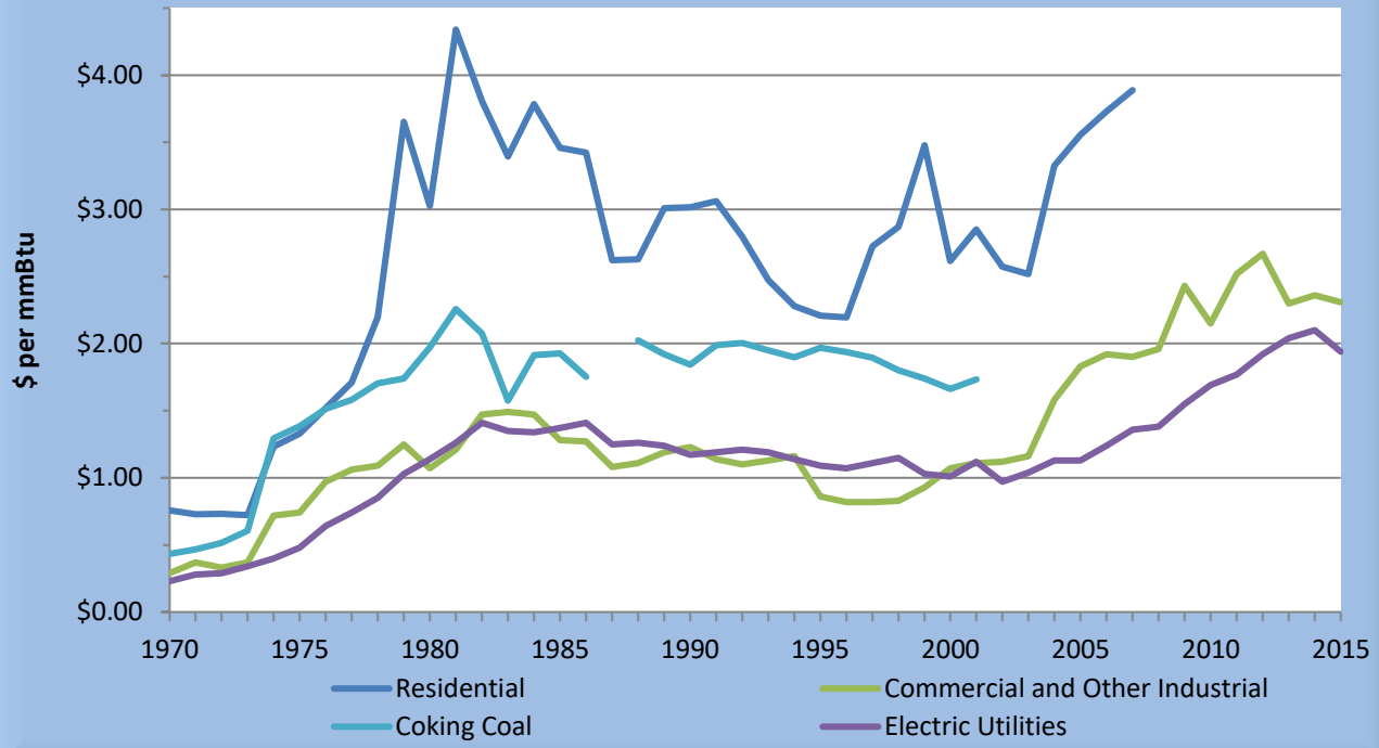
Figure 2.11 - End-Use Price of Coal Consumed in Utah, 1970-2015
